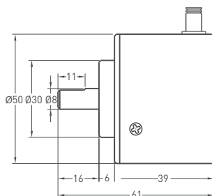
Rod type / Radial cable output
